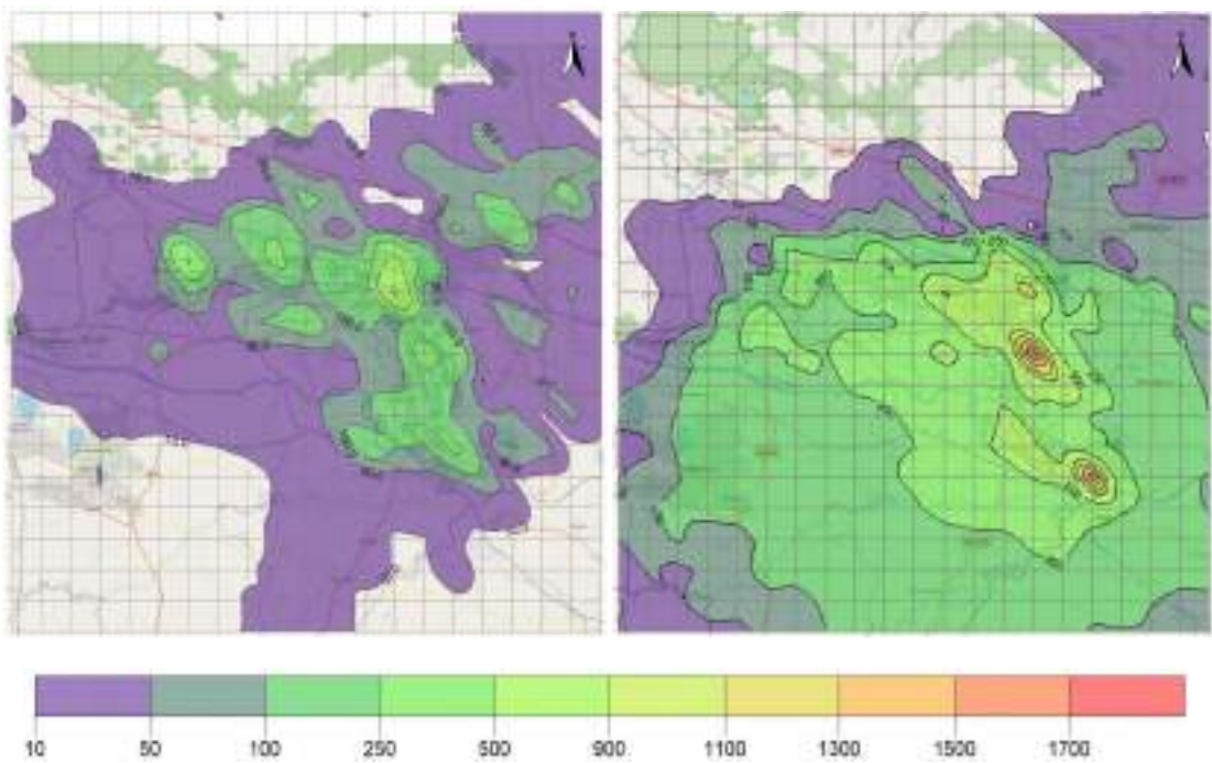
Figure 5.3 (a): 24-hour average maximum ground level concentration of PM 10 (µg/m 3 ) contours in the study area simulated during the study periods in summer (left) and winter (right) seasons.
