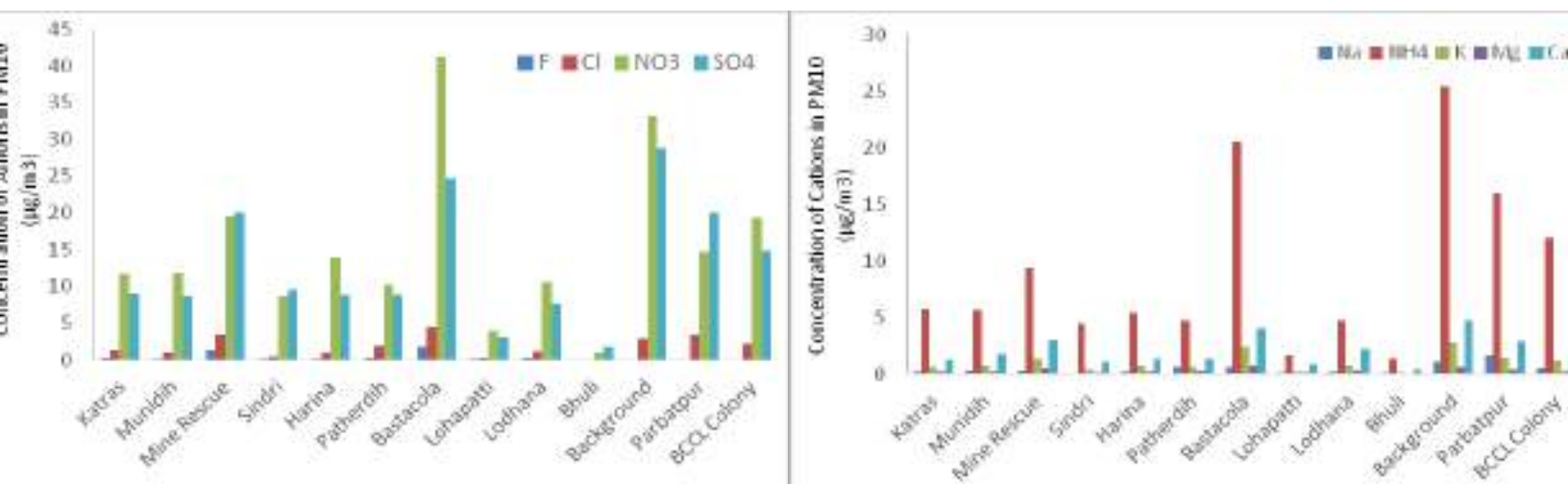
Cation concentration in PM 10 in winter
