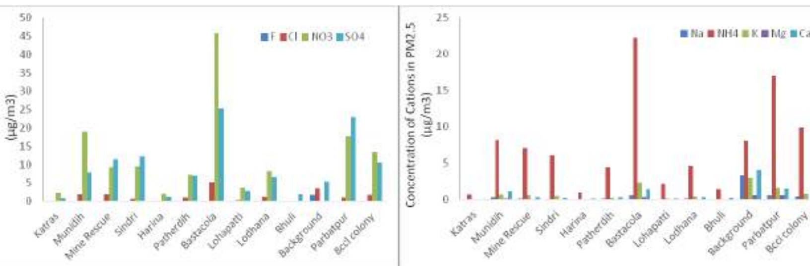
Cation concentration in PM 2.5 in winter
