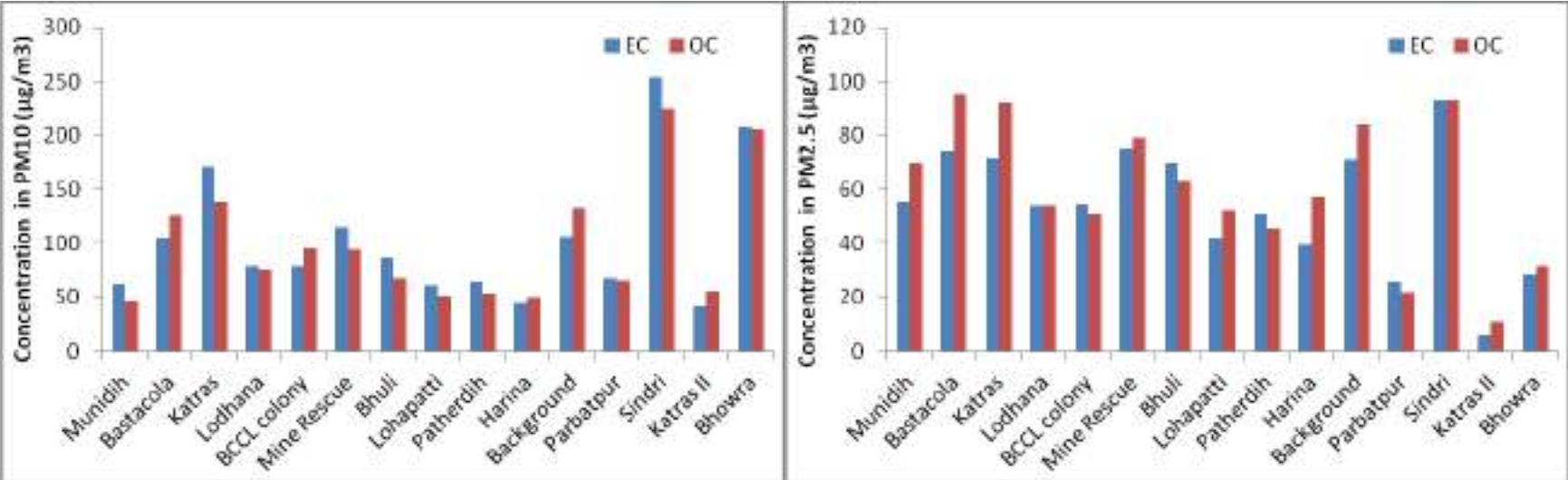
Figure 0.11: EC & OC concentration in PM 10 and PM 2.5 in Winter Season
