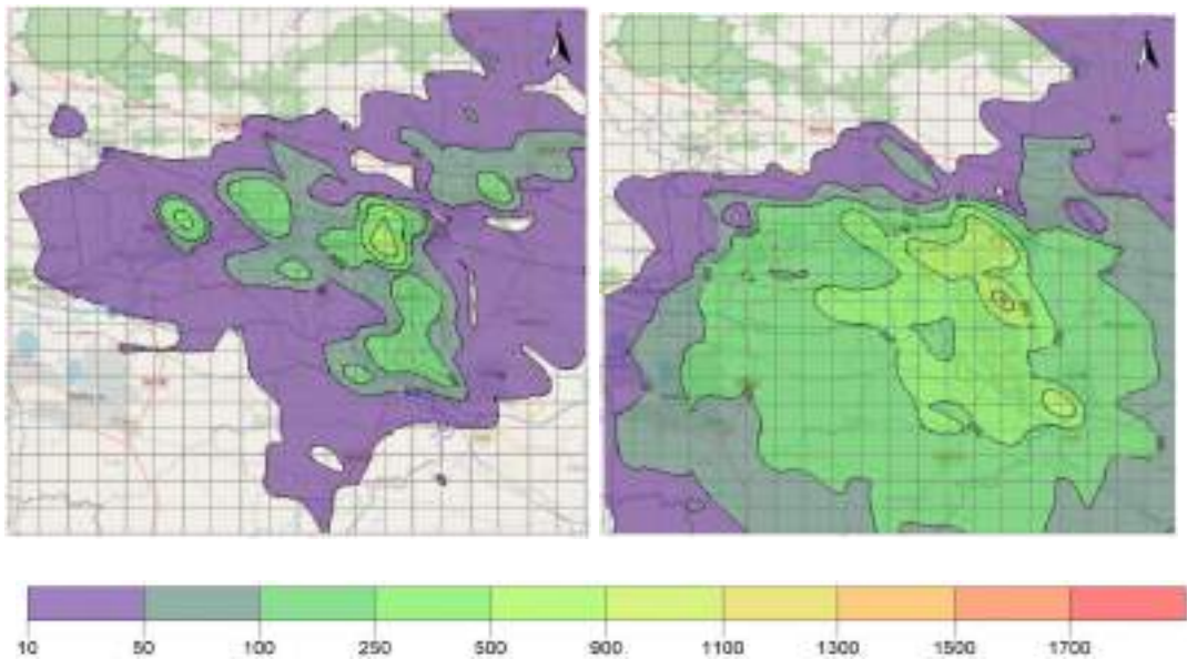
Figure 5.3 (a): 24-hour average maximum ground level concentration of PM 10 (µg/m 3 ) contours in the study area simulated during the study periods in summer (left) and winter (right) seasons.
