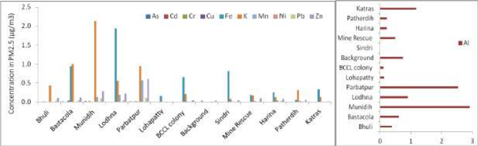
Figure 0.7: Metal concentration of PM 2.5 in winter season
