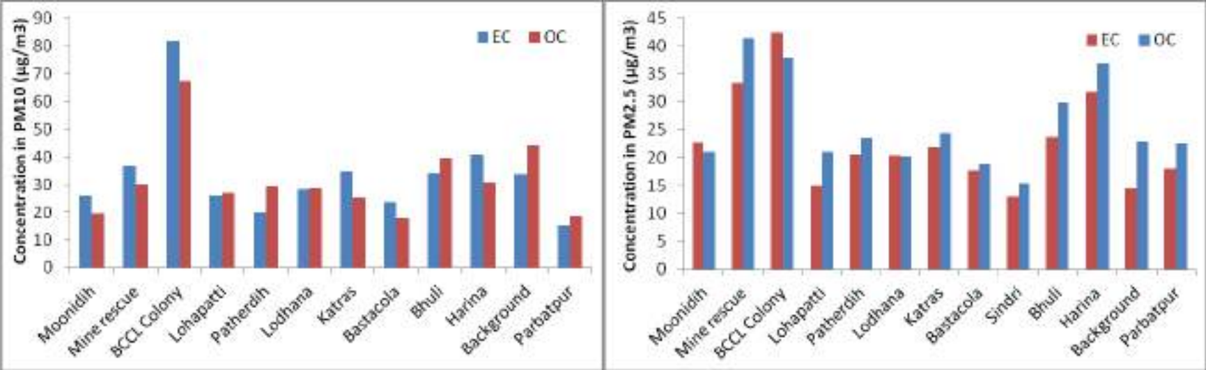
Figure 0.10: EC & OC concentration in PM 10 and PM 2.5 in Summer season
